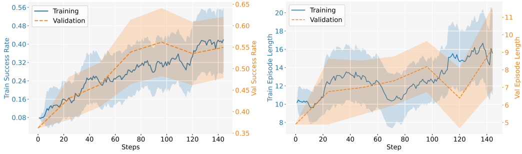
Figure 8: Orchard-Claw RL training curves. Left: train and validation success rate over RL steps. Right: train and validation episode length (number of agent turns per rollout). Validation tasks are sampled from the ClawEval benchmark. Both metrics rise steadily over the course of training, indicating that the agent learns to solve more tasks while also engaging in longer multi-turn interactions.
